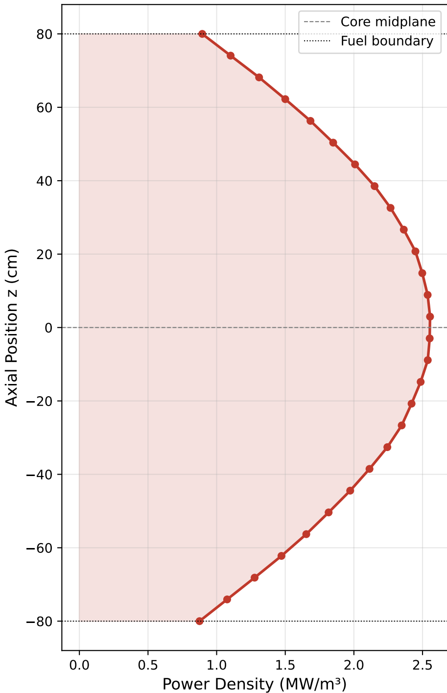
AYURI Core — Axial Power Distribution (normalized to 2.5 MWth)
